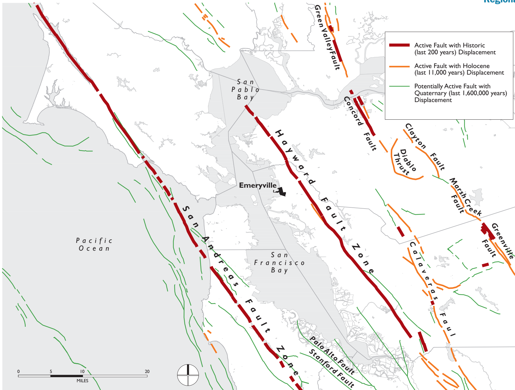
FIGURE 6-3 Regional Faults
