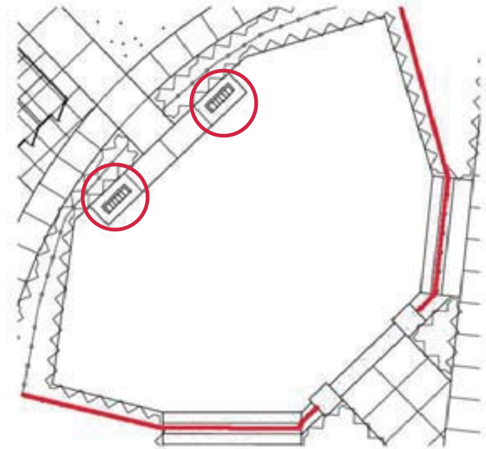
BENCH AND FENCING PLAN FOR PLAY AREA
